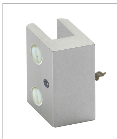
Sign holder with concealed screw connection, silver coloured, anodized with plastic clamping screws
