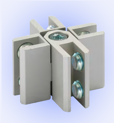
for panel thicknesses of 3 - 8 mm
