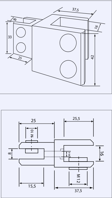
for panel thicknesses of 10 - 16 mm
