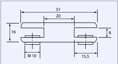
for panel thicknesses of 3 - 10 mm
